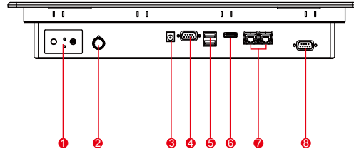
Real Flat Panel Mount (IP65 front side)
