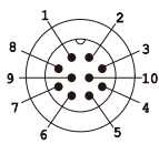
10 pin VGA connector
